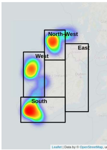
Alexandrium sp.
